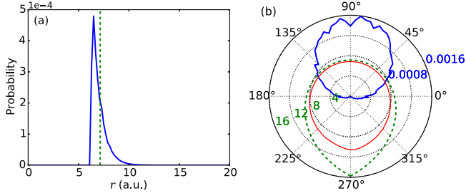
FIG. 3. Electron distributions (blue solid line) as in Fig. 2 but integrated over \tau and all phase-space variables but (a) the distance r to the ion and (b) the angle \theta in the polarization plane. The green dashed lines represent the respective static tunnel exit r_{\text{stat}} . Additionally shown in (b) is the angular distribution of mean tunnel exits from backpropagation (red solid line).
