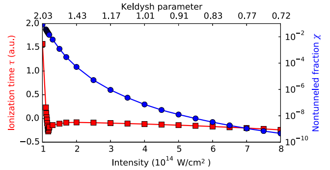
FIG. 4. The fraction of nontunneled electron probability \chi (blue circles) according to Eq. (5) and the mean tunneling ionization time (red squares) for helium as in Fig. 1.
