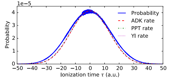
FIG. 1. Distribution (1) of tunneling ionization times [blue solid line, Eq. (1)] for ionization of a SAE helium atom with a laser pulse of 8 \times 10^{14} W/cm 2 peak intensity as described in the text. In comparison, we show related instantaneous rates. For ADK [18,19], we use Eq. (9) of Ref. [19], for PPT [20–23] the equations summarized by Popov [23] [Eqs. (3.4)–(3.6)], and for YI the circular case in Yudin and Ivanov [24] [Eqs. (19) and (20)]. All rates are scaled to agree at the maximum.
