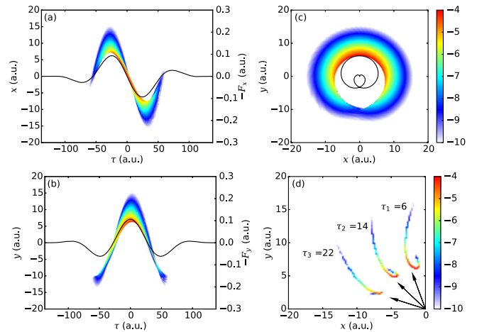
FIG. 2. Distributions d^3\mathcal{P}/drd\tau (in logarithmic scale) of the tunneling ionization time \tau and position (x, y) according to Eq. (1) for the system as in Fig. 1 projected onto the planes (a) \tau - x , (b) \tau - y , (c) x - y , respectively, and (d) sliced at times \tau_i as indicated. Black lines or arrows indicate the electric field at times t = \tau , (a) -F_x (in a.u.), (b) -F_y (in a.u.), (c) and (d) -F (in arb. units).
