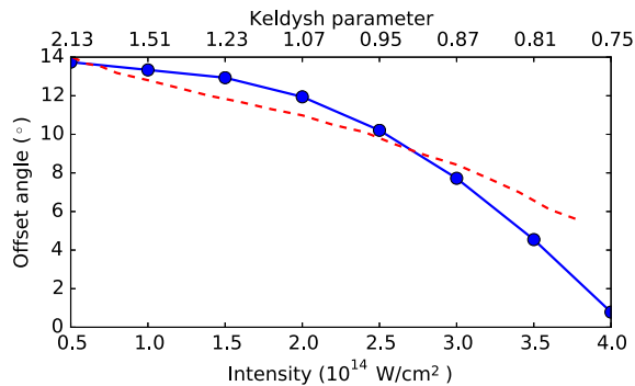
FIG. 6. Intensity dependence of the electron emission angle perpendicular to the direction of maximal field strength of the light pulse for hydrogen as in Fig. 5. The red dashed curve is the corresponding angle from Ref. [9].
