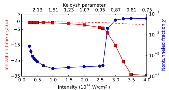
FIG. 5. The fraction of nontunneled ionization probability \chi (blue circles) according to Eq. (5) and the mean tunneling ionization time (red squares) as in Fig. 4 but for hydrogen with potential V(r) = -(r^2 + 0.63629)^{-1/2} . The red dashed curve is the ionization time from Ref. [9].
