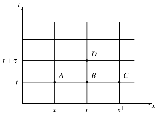
Fig. 1. The difference stencil in the tx plane.
