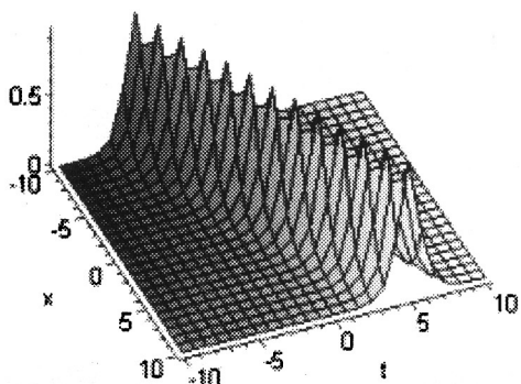
Fig. 6. Solution (4.13) with parameters a_1 = 1 , a_2 = 6 , a_3 = -1 , p = 4 , \beta = 2 .
