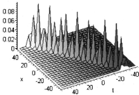
Fig. 2. Imaginary part of solution (3.23) with parameters A_0 = 1, a_1 = 4, a_2 = 1, a_3 = -1, p = 2, \beta = 2, \gamma = 1 .
