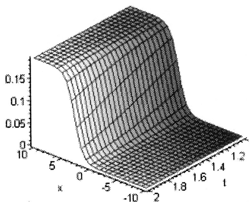
Fig. 1. Real part of solution (3.23) with parameters A_0 = 1, a_1 = 4, a_2 = 1, a_3 = 1, p = 2, \beta = 2, \gamma = 1 .
