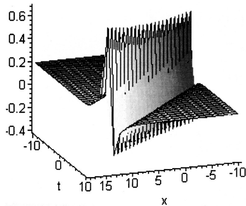
Fig. 4. Solution (3.28) with parameters A_0 = 1, a_1 = 4, a_2 = 1, a_3 = -1, p = 2, \beta = 2, \gamma = 1 .
