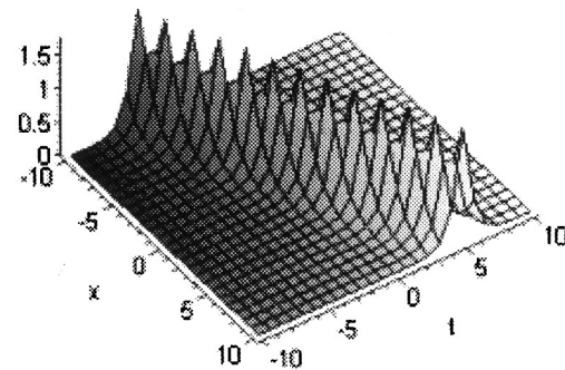
Fig. 5. Solution (3.37) with parameters a_1 = 1, a_2 = -1, p = 3, \beta = 2 .
