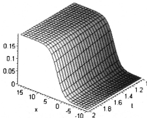
Fig. 3. Solution (3.27) with parameters A_0 = 1, a_1 = 4, a_2 = 1, a_3 = -1, p = 2, \beta = 2, \gamma = 1 .
