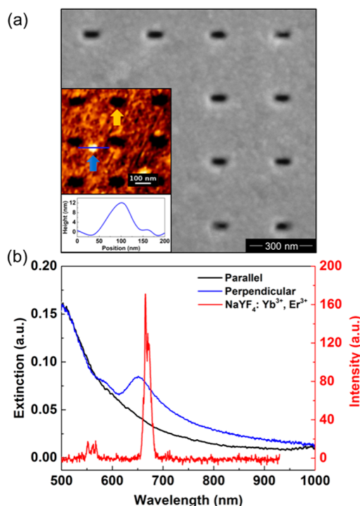
Figure 1. (a) SEM image of rectangular slot nanoantenna array. Inset: AFM topographic image of NaYF 4 :Yb 3+ , and Er 3+ nanoparticles on the nanoantenna array and the line scan. The blue and yellow arrows indicate the single UCNP and the rectangular slot, respectively. (b) Measured extinction spectrum of the nanoantenna array under the plane-wave illumination with the polarization parallel and perpendicular to the long axis of the slots and the UCL spectrum of NaYF 4 :Yb 3+ , and Er 3+ nanoparticles on glass coverslip.
