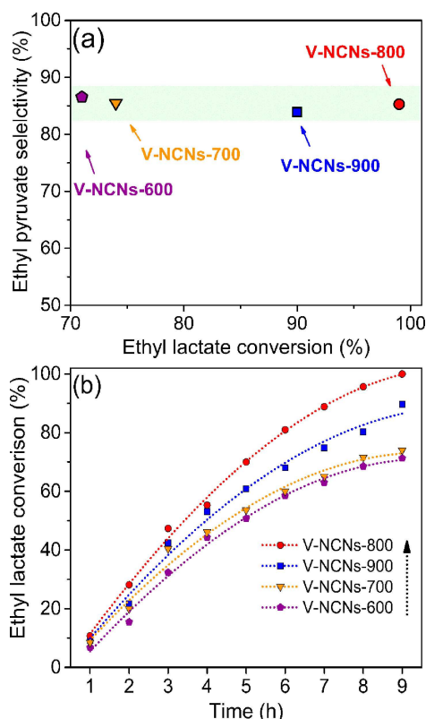
Figure 3. (a) Comparisons of the aerobic oxidation of ethyl lactate to ethyl pyruvate over the various V-NCNs- x catalyst. Reaction conditions: ethyl lactate 5 mmol, catalyst 25 mg, 1 atm O 2 , diethyl succinate (solvent, 1 ml), molecular sieve-3 Å (dehydrating agent, 100 mg), 130 °C and 9 h. (b) The time-resolved conversion profile of ethyl lactate over the V-NCNs- x catalysts.
