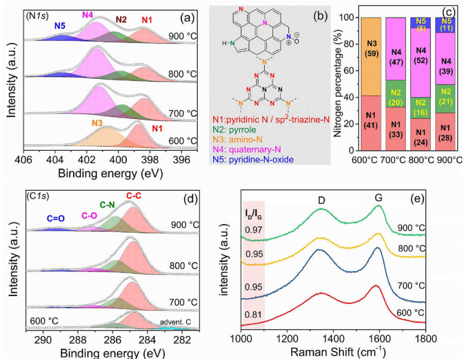
Figure 4. (a) XPS spectra of N 1s in the V-NCNs- x catalysts ( x = 600, 700, 800 and 900 °C) (b) types of nitrogen functionalities occurring in V-NCNs- x samples and (c) nitrogen contents of NCNs- x with different pyrolysis temperatures (N1: sp 2 hybridized-N, red; N2: pyrrolic-N, green; N3: amino-N, yellow; N4: graphitic-N, pink; N5: pyridine oxide-N, blue). The nitrogen species were quantified based on XPS data of the materials treated at different temperatures. (d) high-resolution C 1s spectra of V-NCNs- x . (e) Raman spectra of V-NCNs- x samples.
