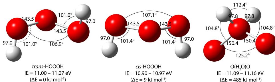
Fig. 1. CCSD(T)/aug-cc-pVTZ optimized geometries of \text{H}_2\text{O}_3 isomers. Bond lengths and angles are in the units of picometers (pm) and degrees ( ^\circ ), respectively, while relative energies with respect to trans -HOOOH ( \Delta E ) are given in the units of kilojoules per mole ( \text{kJ mol}^{-1} ). Corresponding adiabatic IEs are provided in electron volts (eV).
