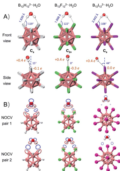
Fig. 2 (A) Lowest-lying structures of B_{12}X_{12}^{2-} \cdot H_2O ( X = H, F, I ) with the corresponding bond lengths, bond angles of B–X···H, dihedral angles between X–B–X and H–X–H planes, and restrained electrostatic potential charge (RESP charge) of X atoms and H atoms in H_2O . (B) Plot of electron density changes of two dominant ETS-NOCV pairs arising from orbital interactions between B_{12}X_{12}^{2-} ( X = H, F, I ) and H_2O with an isovalue of 0.0007 a.u.
