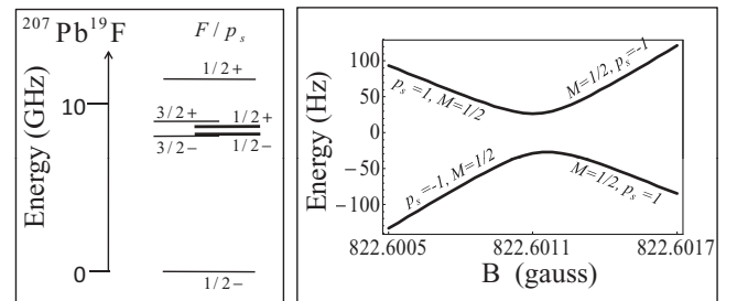
FIG. 1. Left hand side: Hyperfine energy level structure of the ground electronic ( X_1 ) and rotational ( J = 1/2 ) state of the 207 Pb 19 F molecule as a function of F (total angular momentum) and p_s (parity). Two closely spaced F = 1/2 states of opposite parity are shown by thick lines. Right hand side: Anapole-induced avoided crossing of the M_F = 1/2 sublevels of the closely spaced M_F = 1/2 states. This crossing is predicted to occur at a field of 823 \pm 40 G.
