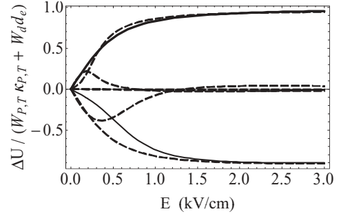
FIG. 2. P - and T -odd dependent splitting between \pm M_F pairs of hyperfine states of the ground rotational J = 1/2 state of ^{207}\text{Pb}^{19}\text{F} . The thick solid line corresponds to the |M_F| = 3/2 lower lying \Omega -doublet states whereas the thin solid line corresponds to the higher lying |M_F| = 3/2 states. The dotted lines correspond to |M_F| = 1/2 sublevels. For the case that \kappa_{P,T} = 0 and d_e = 1.6 \times 10^{-27} e·cm (the current limit of Ref. [5]), the energy scale is 26 mHz.
