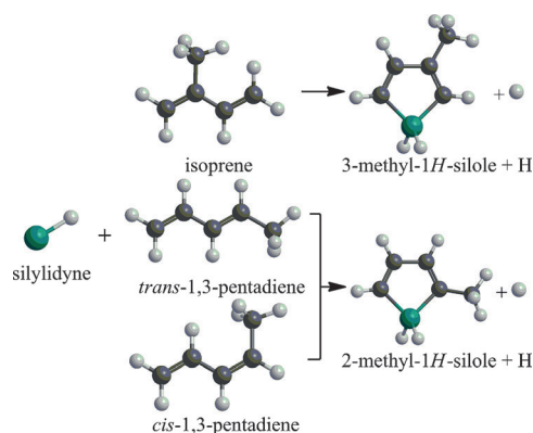
Scheme 2. Potential pathways for the formation of singly substituted siloles through the reaction of silyldiyne with alkyl-substituted 1,3-butadienes, such as isoprene and 1,3-pentadiene, in the gas phase.
