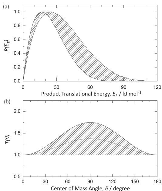
Figure 2. a) The center-of-mass translational energy distribution, P(E_T) , and b) the angular distribution, T(\theta) , for the reaction of the silyldiyne radical with 1,3-butadiene forming \text{SiC}_4\text{H}_6 isomer(s) by atomic hydrogen emission. The hatched areas indicated the experimental error limits.
