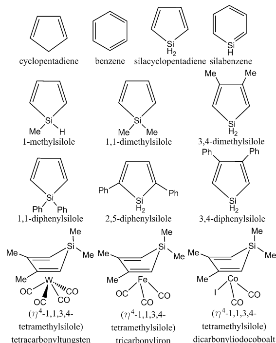
Scheme 1. Structures of prototype cyclic hydrocarbons and their silicon analogues, mono-, dimethyl-, and diphenyl-substituted siloles, as well as metal complexes of \eta^4 -siloles indicating the roles of siloles as ligands with transition metals.
