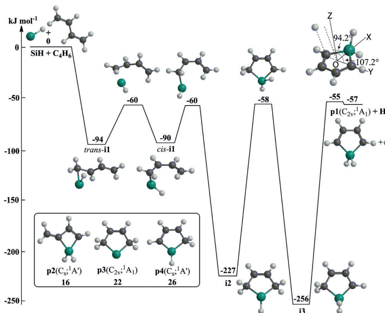
Figure 3. Potential energy surface of \text{SiC}_4\text{H}_7 for the reaction of the silyldiyne radical with 1,3-butadiene leading to p1 (silole; c- \text{SiC}_4\text{H}_6 ) and atomic hydrogen. Three energetically accessible product isomers, p2–p4 , are shown along with the point groups and symmetries of the electronic wave functions. The energies are given in \text{kJ mol}^{-1} with respect to the initial reactant system. Carbon black, hydrogen light gray, silicon dark green.
