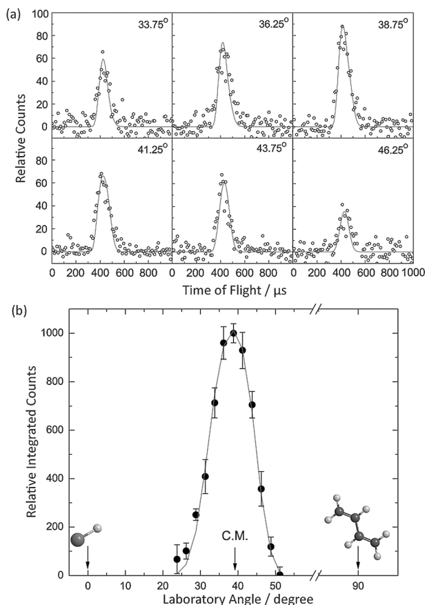
Figure 1. a) Time-of-flight spectra and b) laboratory angular distribution recorded at m/z 82 ( \text{SiC}_4\text{H}_6^+ ) for the reaction of the silyldiyne radical with 1,3-butadiene. The circles represent the experimental data points while the solid lines represent the best fits.
