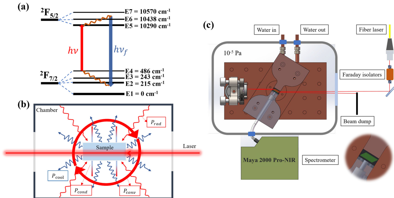
FIG. 1. (a) The Stark sublevel energy diagram for Yb 3+ ions 53 (not to scale) in LuLiF 4 involving absorption (red arrow), anti-Stokes emission (blue arrow), and phonon relaxation (orange arrows). (b) The heat load from three main sources: the convective heat load P_{conv} , the conductive heat load P_{cond} , and the blackbody radiative heat load P_{rad} . (c) Schematic of the experimental setup. A partial enlargement of the clamshell containing the sample is shown in the right corner.
