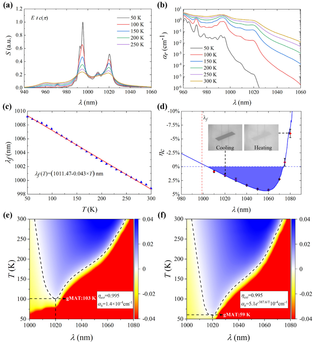
FIG. 2. (a) Temperature-dependent fluorescence spectra of \text{Yb}^{3+}:\text{LuLiF}_4 crystal ( E||c ). (b) The absorption spectrum \alpha_r(\lambda, T) obtained from the fluorescence spectrum ( E||c ) according to the reciprocity relationship. (c) Dependence of the mean fluorescence wavelength on the sample temperature. (d) The LITMoS test results and the fitting curve \eta_c(\lambda, T) for the 7.5% \text{Yb}^{3+}:\text{LuLiF}_4 crystal. The insets show the thermal images of the sample at 1020 and 1080 nm excitation, respectively. (e) Cooling efficiency contour map \eta_c(\lambda, T) for the 7.5% \text{Yb}^{3+}:\text{LuLiF}_4 crystal. Blue region denotes cooling, and red region denotes heating. (f) Cooling efficiency contour map \eta_c(\lambda, T) for the 7.5% \text{Yb}^{3+}:\text{LuLiF}_4 crystal in light of the background absorption as a function of the sample temperature.
