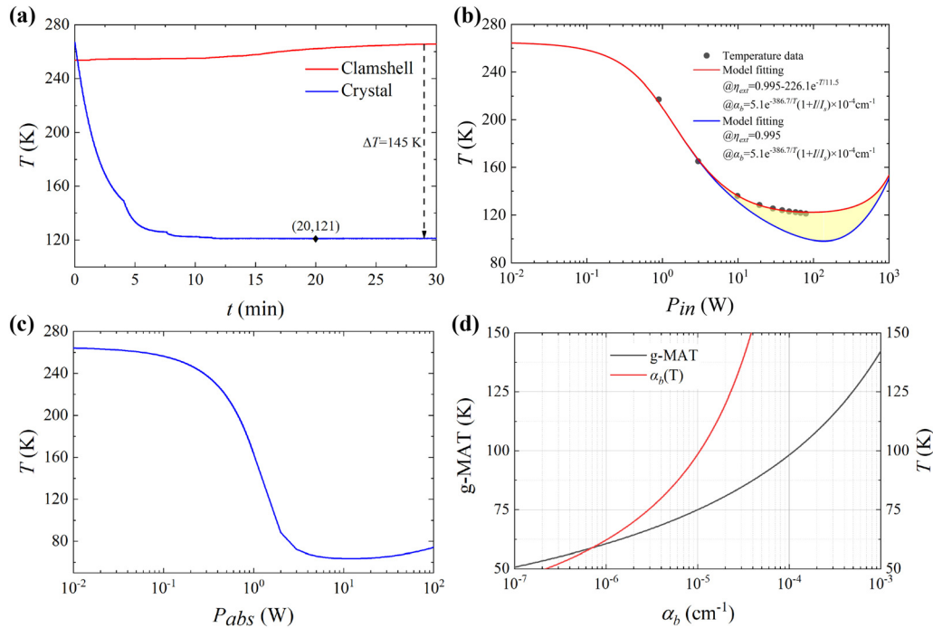
FIG. 3. (a) Time-dependent temperature evolution of the crystal. (b) The measured steady-state temperature of the crystal under different pump laser power and model fitting using Eq. (2) with I_s = 11.45 \text{ kW/cm}^2 . The yellow region indicate that the water condensation effect plays an important role on the final steady-state temperature of the sample. (c) The cooling temperature from model fitting using Eq. (2) vs absorbed pump laser power considering the saturation absorption effect. (d) Dependence of the effective background absorption on the sample temperature and the g-MAT of the sample predicted from the theoretical model.
