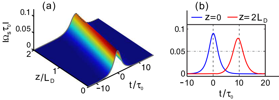
Fig. 2. (a) The propagation of the ultralow optical soliton, with |\Omega_s(z, \tau)\tau_0| as a function of z/L_D and t/\tau_0 ( L_D is dispersion length and \tau_0 is pulse duration). (b) The comparison of waveshapes between z = 0 (blue curve) and z = 2L_D (red curve).
