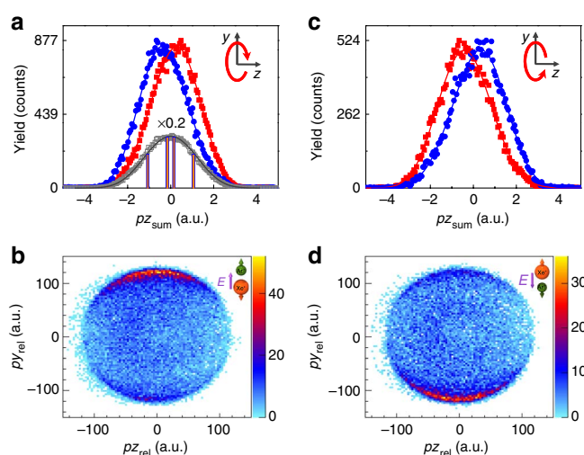
Figure 3 | Ion sum- and relative-momentum distributions of \text{Ar}^+ + \text{Xe}^+ breakup. (a,c) Ion sum-momentum distributions. These reflect the recoil of two sequentially emitted electrons. The red squares and blue circles are events where \text{Ar}^+ fly in the +y and -y directions, and the grey squares are the sum of them. To guide the eye, four possible sum momenta of the sequentially ionized electrons are indicated by the pink bars in (a) under the grey curve. (b,d) Ion relative-momentum distributions. These reflect the \text{ArXe} orientation. Only the events when the instantaneous field vector (violet arrow) at the release of the second electron pointing along (b) +y , or (d) -y , are selected by choosing p_{z_{\text{sum}}} > 1.0 a.u. (see text for details). In agreement with the intuitive picture of the enhanced ionization, the second electron from \text{ArXe} is favoured to be freed when the instantaneous laser field is pointing from \text{Xe}^+ towards the \text{Ar} atom. As sketched by the inset red ellipses at the top-right corners of (a) and (c), the sense of rotation of the electric field vector of our laser pulse is adjusted to be (a,b) clockwise, and (c,d) anticlockwise, respectively. The unit for the colour scale is counts.
