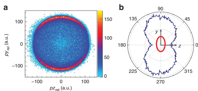
Figure 2 | Relative momentum and angular distributions of \text{Ar}^+ + \text{Xe}^+ breakup. (a) Measured relative momentum distribution between \text{Ar}^+ and \text{Xe}^+ from Coulomb exploding double ionization of \text{ArXe} using elliptically polarized femtosecond laser pulses whose major and minor axes are orientated along y - and z -axis, respectively, as sketched by the red ellipse in (b). (b) The corresponding angular distribution of the \text{Ar}^+ + \text{Xe}^+ breakup in the polarization plane of the laser pulse. The double-ionization rate maximizes for molecules orientated along the polarization major axis of our elliptically polarized laser field. The unit for the colour scale is counts.
