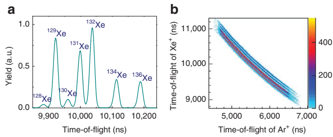
Figure 4 | Two-particle correlation identifies ArXe isotopes. (a) Measured time-of-flight mass spectrum of the \text{Xe}^+ isotopes. (b) Correlations between the times-of-flight of the Coulomb exploding \text{Ar}^+ and \text{Xe}^+ following two-side double ionization of ArXe. Each sharp stripe stands for one ArXe isotope. The unit for the colour scale is counts.
