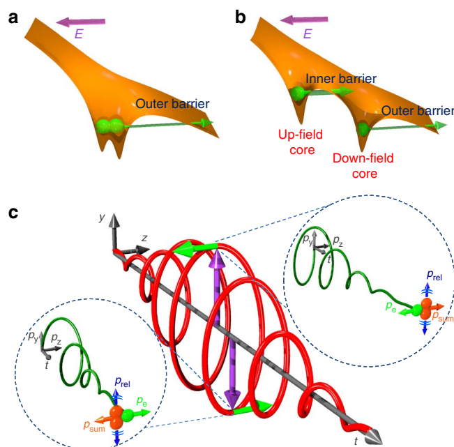
Figure 1 | Enhanced ionization scenario and the angular streaking concept.
