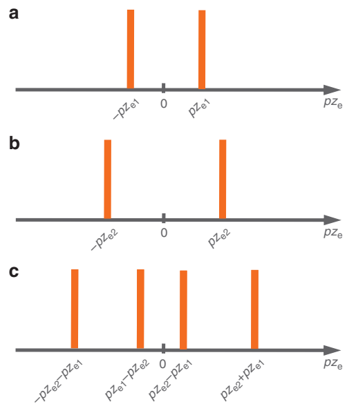
Figure 5 | Schematic illustration of the momentum convolution of two sequentially released electrons. The orange bars indicate the momentum peaks of the (a) first and (b) second electrons, and (c) the eventually measured distribution as a result of their convolution.
