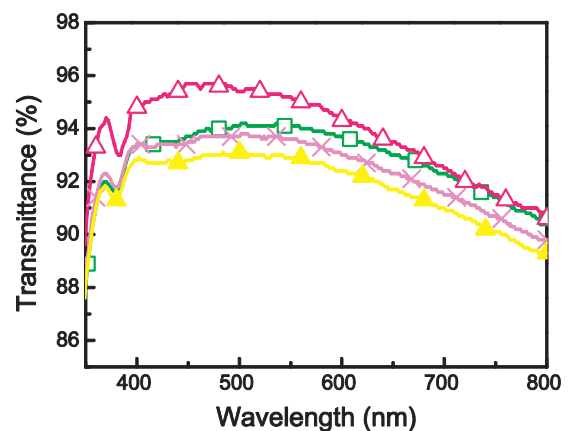
Fig. 5. Transmission spectra of glass slides with Ag/SiO 2 coatings with the thicknesses of 135 nm (□), 120 nm (Δ), 87 nm (×), 52 nm (▲).
