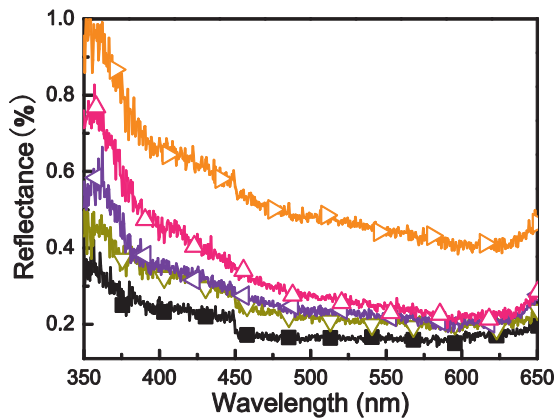
Fig. 3. Reflection spectra of glass slides with Ag/SiO 2 coatings with Ag concentration of 0.10 wt.% (Δ), 0.05 wt.% (◁), 0.025 wt.% (▽), 0.20 wt.% (▷), and pure glass slide (■).
