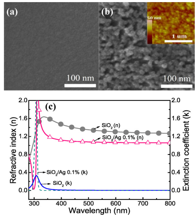
Fig. 4. SEM images of top morphology on glass slides coated with pure SiO 2 (a) and Ag/SiO 2 film with Ag concentration of 0.1 wt.% (b) (inset of figure (b): AFM image of Ag/SiO 2 coating). (c) Refractive index and extinction coefficient of pure silica film and Ag/SiO 2 film with Ag concentration of 0.1 wt.%.
